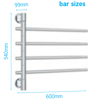
Vertical and horizontal bar sizes
